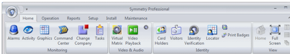
Figure 2-2: Ribbon Bar
