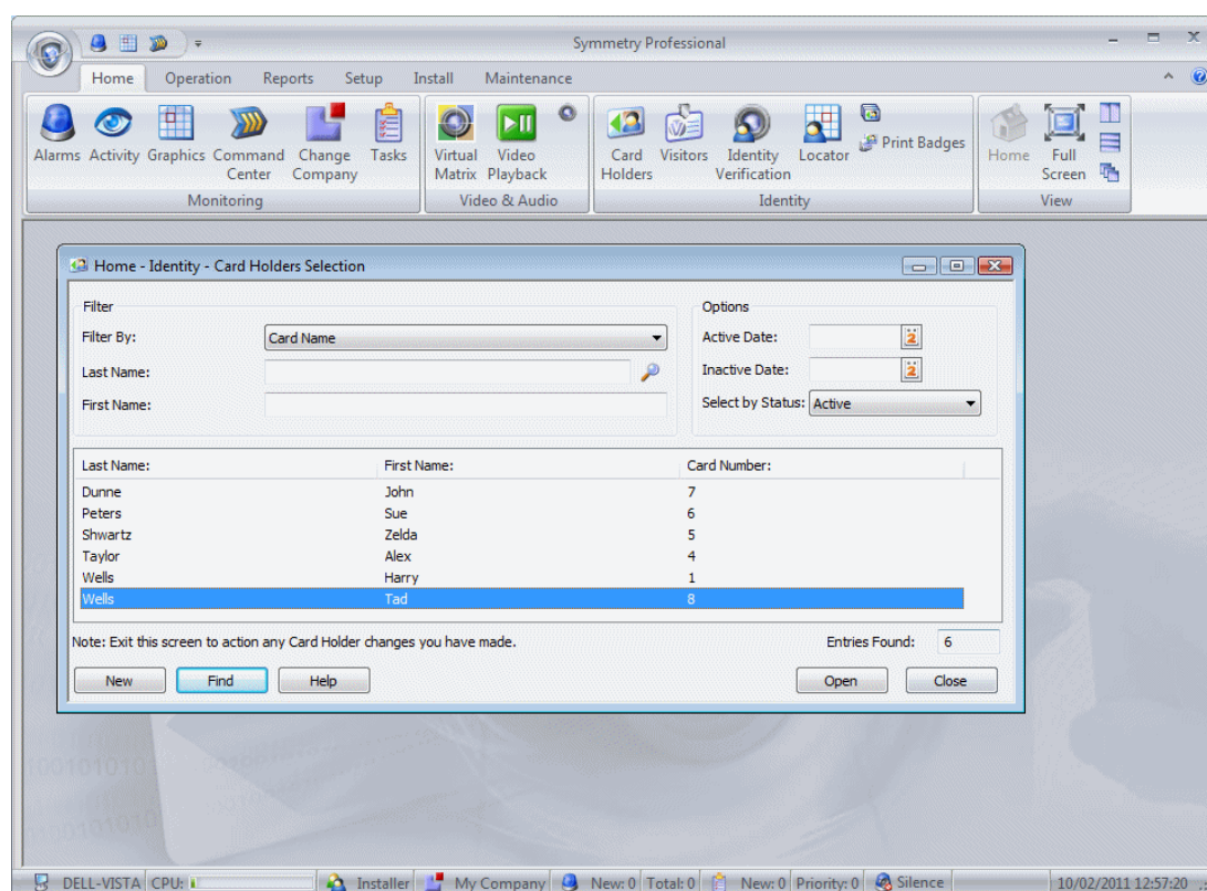
Figure 1-1: Symmetry Software
